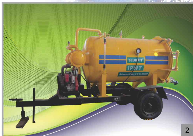
1. Mini-size trailer-mounted SLURPIT® suction unit (1500 ltrs) ; supplied to Shimoga City Municipal Council in 2000
